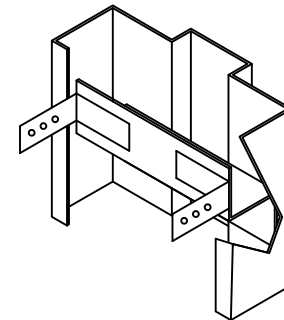
WSC W/ WSA ANCHOR DETAIL
