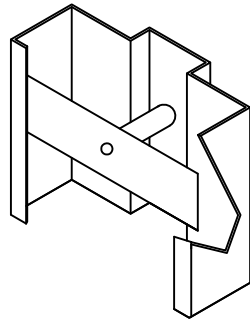
EXISTING WALL ANCHOR (EWA) DETAIL
