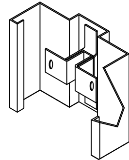
COMPRESSION BAR ANCHOR (CBA) DETAIL
