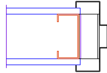
RECESSED TYPE - WELDED STEEL STUD ANCHOR
