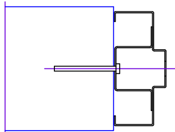
HAT ANCHOR W/ BOLT OR SCREW
