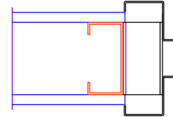
FLUSH TYPE - WELDED STEEL STUD ANCHOR
